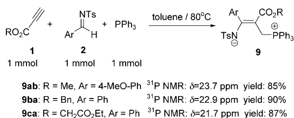
Scheme 8. Formation of the phosphonium–enamine zwitterions; Bn = benzyl.
